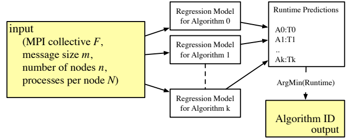
Fig. 3: General algorithm selection strategy for MPI collectives. The running time of each algorithm ( 1 \dots k ) is predicted for a given instance (F, m, n, N) . The algorithm with the smallest predicted runtime is selected.
