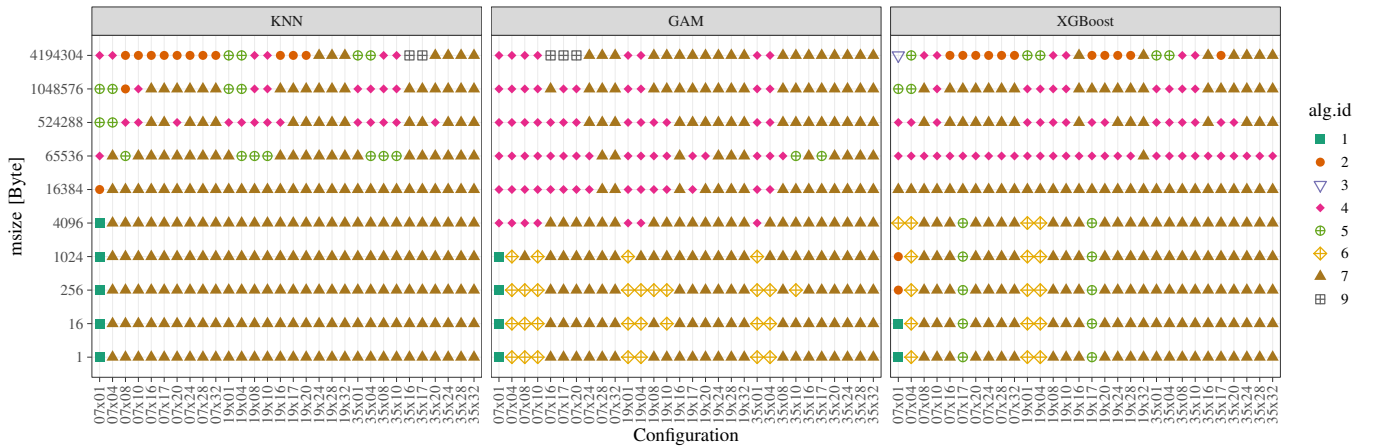
Fig. 5: Overview of the predicted algorithm for various process configurations ( \#nodes \times ppn ) for MPI_Bcast with each of the regression learners; Open MPI 4.0.2; Hydra .
