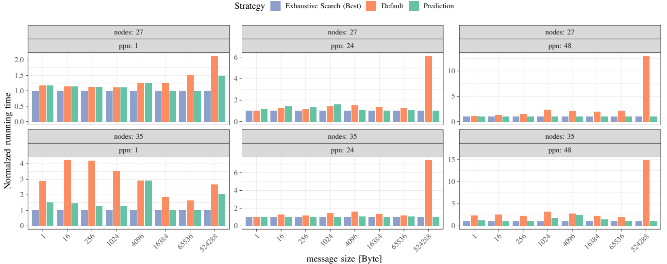
Fig. 8: Comparison of the algorithm selection strategies for MPI_Bcast; Open MPI 4.0.2; SuperMUC-NG.
